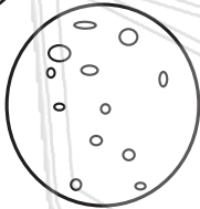
Mercury
