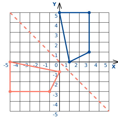
Reflection: Across Line y = -x
