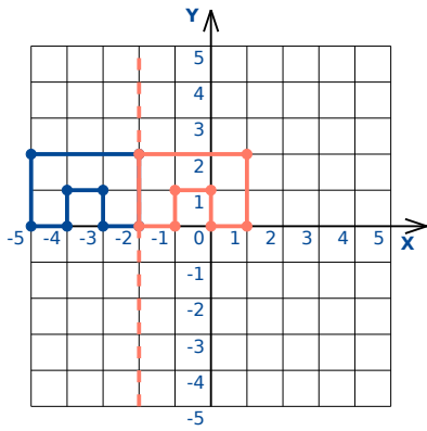
Reflection: Across the line x = -2
