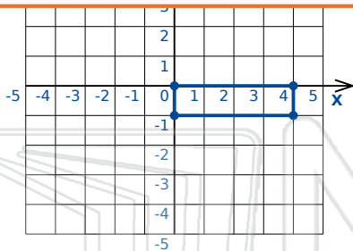
Translation: 4 left and 4 up
