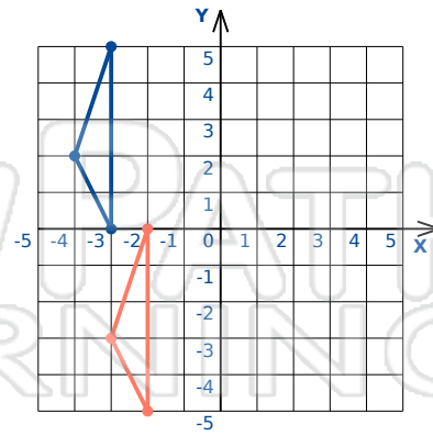
Translation: 1 right and 5 down
