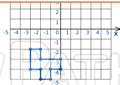
Rotation: 90^\circ clockwise about the origin
